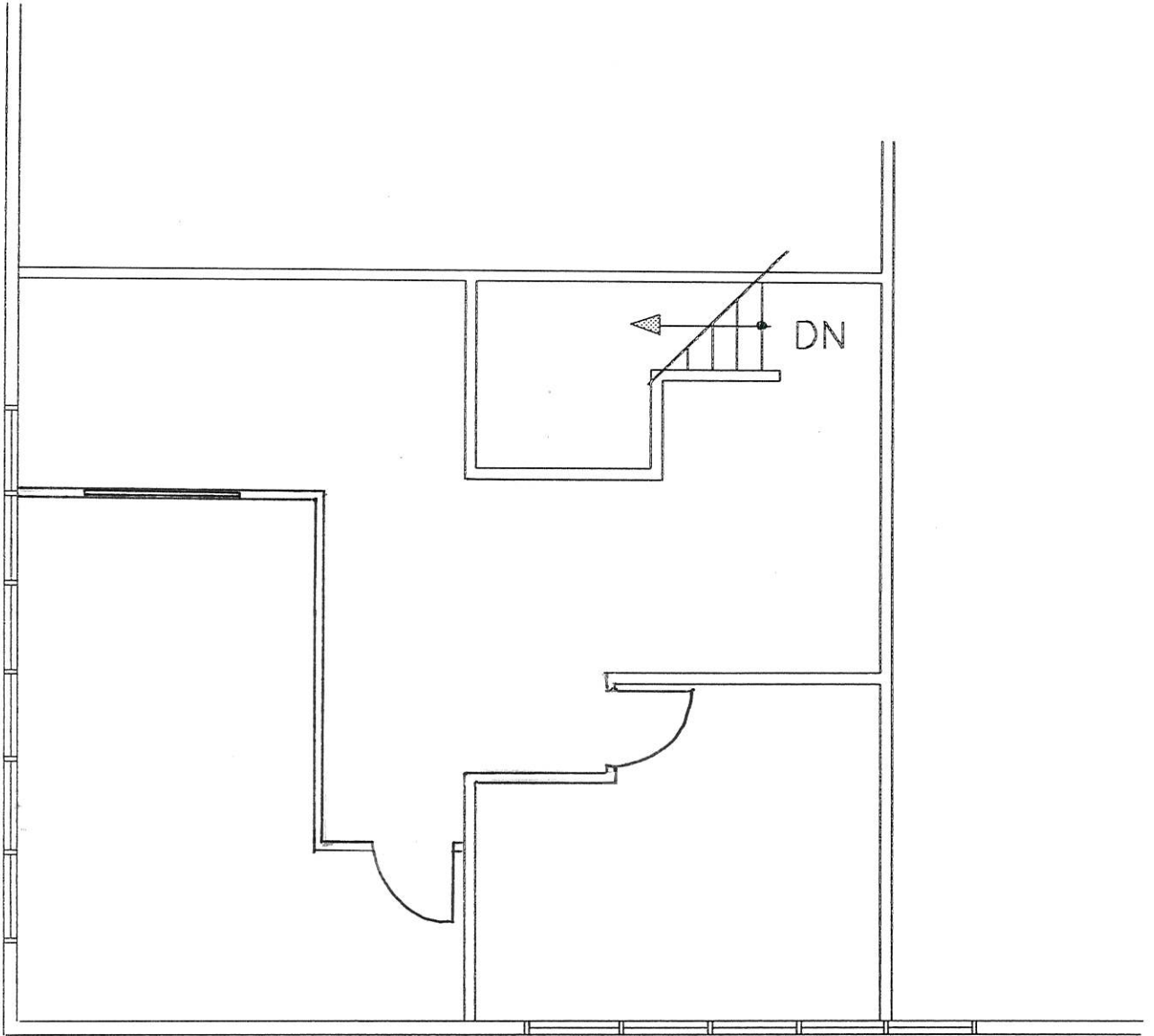
3822 SECOND FLOOR PLAN
