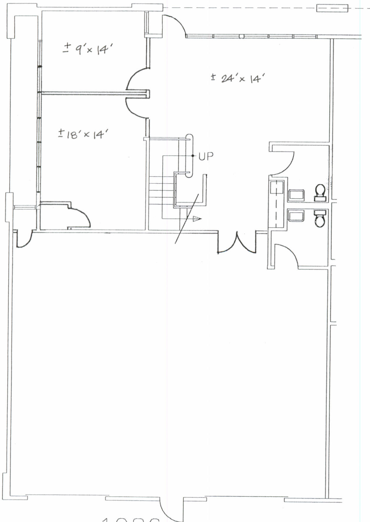
1086 FIRST FLOOR PLAN
