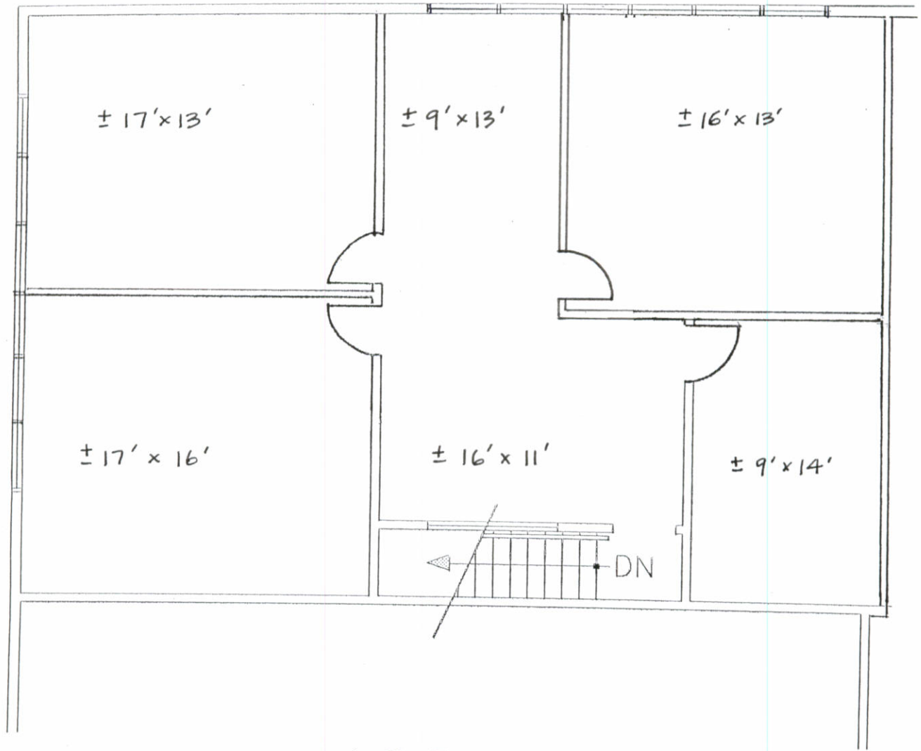
1086 SECOND FLOOR PLAN
